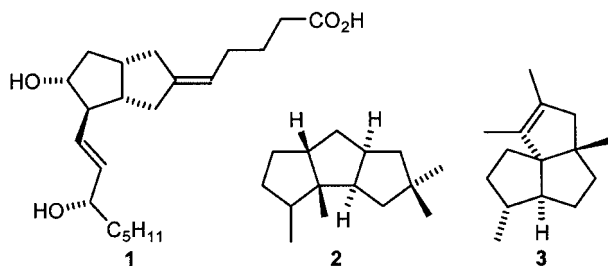
Scheme 1. The bicyclo[3.3.0]octane structural motif in carbacyclin ( 1 ) and the triquinanes hirsutane ( 2 ) or silphiperfolene ( 3 ).
